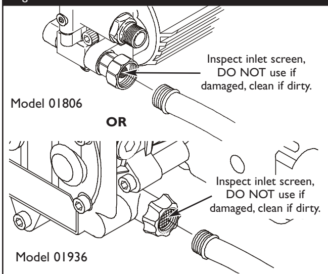
Figure 12 — Connect the Garden Hose to Water Inlet
