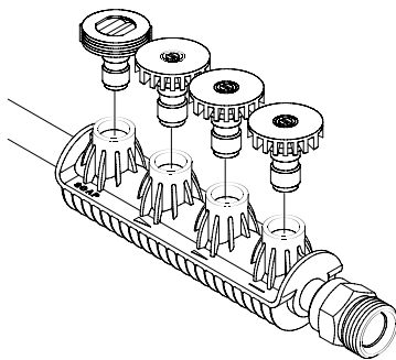
Figure 13 — Install Spray Tips in Holder
